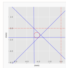
Figure 11: Collimator Spoke Test Report
