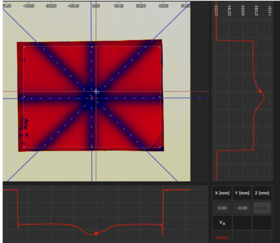
Figure 8: Couch Spoke Test
