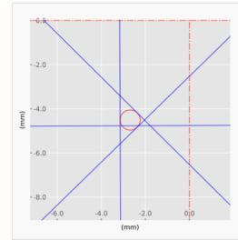
Figure 9: Couch Spoke Test Report
