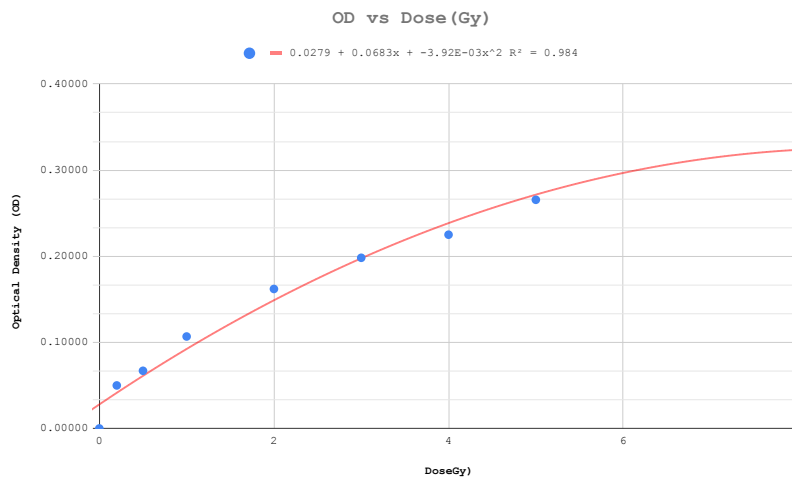
Figure 6: Dose vs Optical Density (OD)
