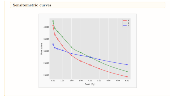
Figure 5: Sensitometric curves
