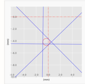
Figure 13: Gantry Spoke Test Report
