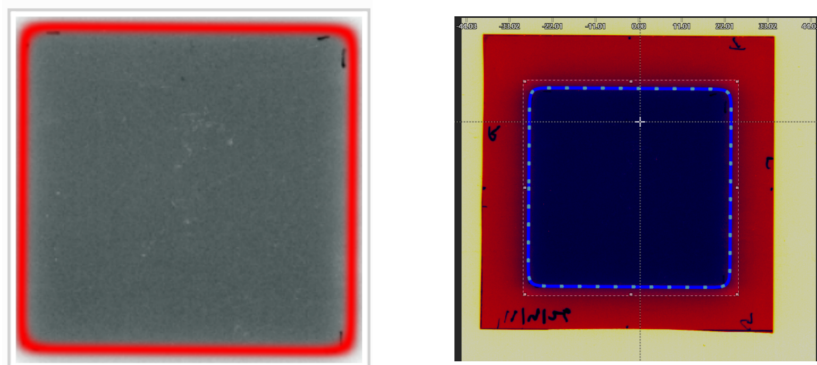
Figure 21: Radiation Field Analysis
